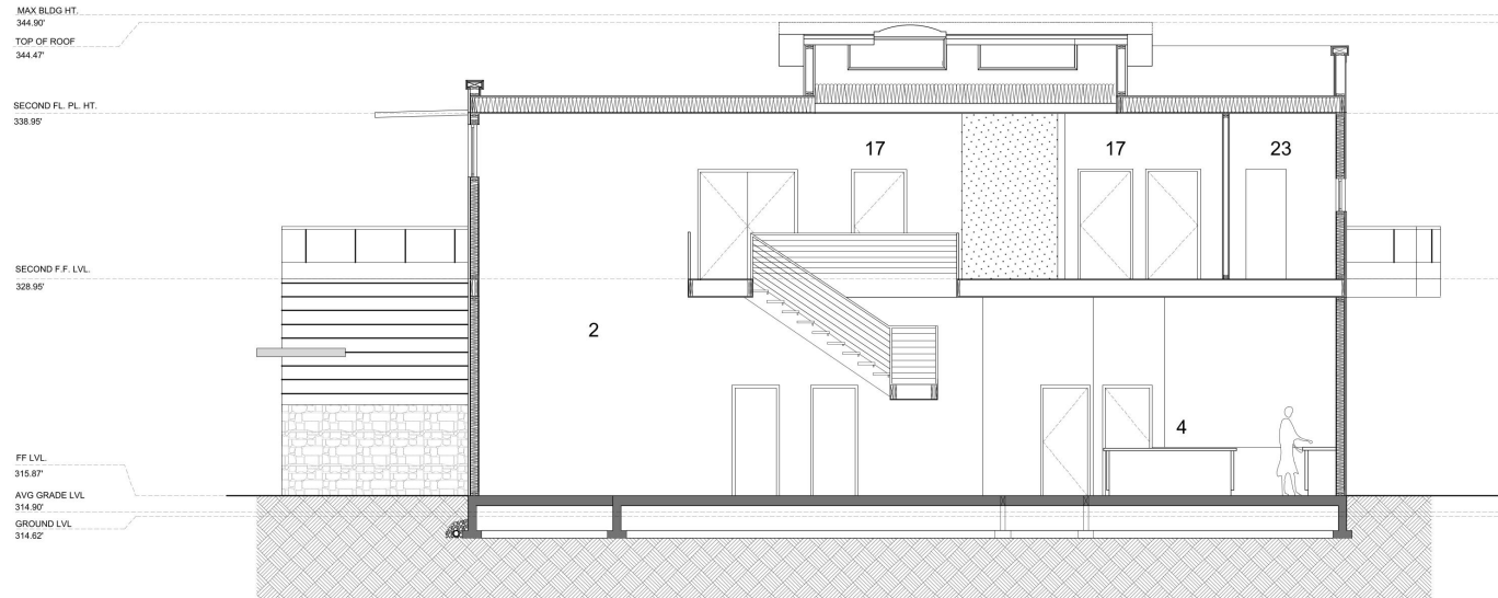
SECTION THROUGH KITCHEN & GARAGE
