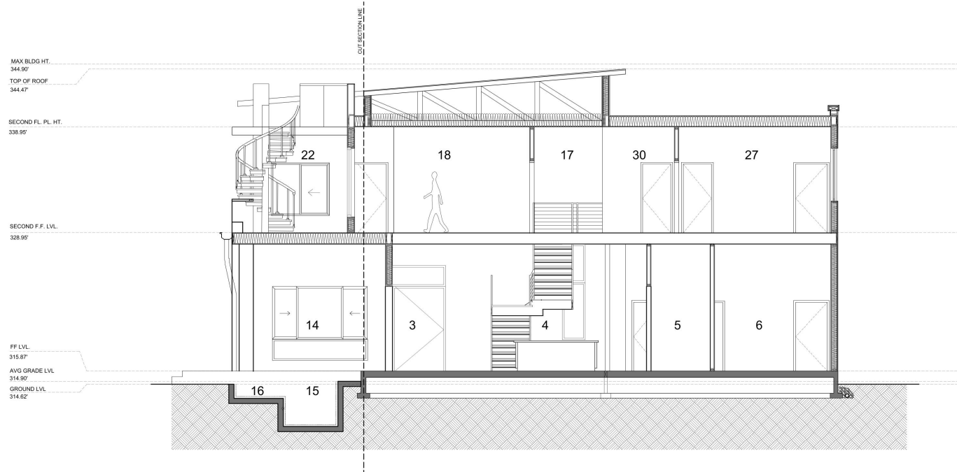
LIVING & DINNING SECTION THROUGH STAIRCASE
